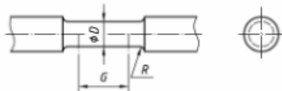
c) Round bar specimen
