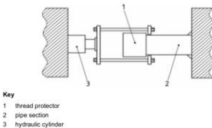
Figure D.26—Stripping Test Apparatus
