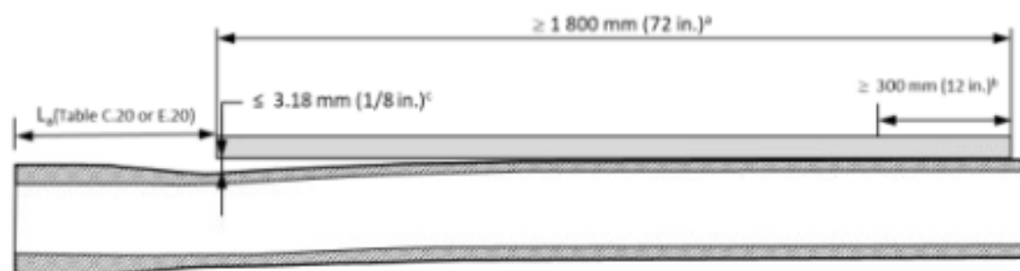
Figure D.15—Gag Straightening Fiber Strain Factors
