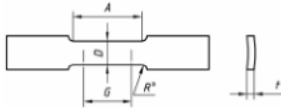
b) Strip specimen a
