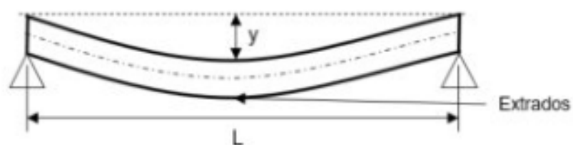
Figure D.15—Gag Straightening Fiber Strain Factors
