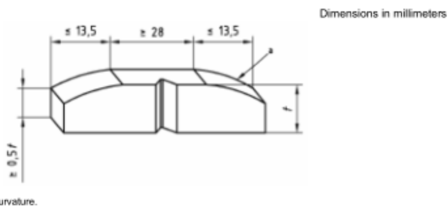
Figure D.12—Charpy Specimen Dimensions
