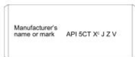
Stencil Marking
