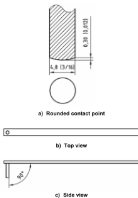
Figure D.23—Example of a 90° Hook-type Tool
